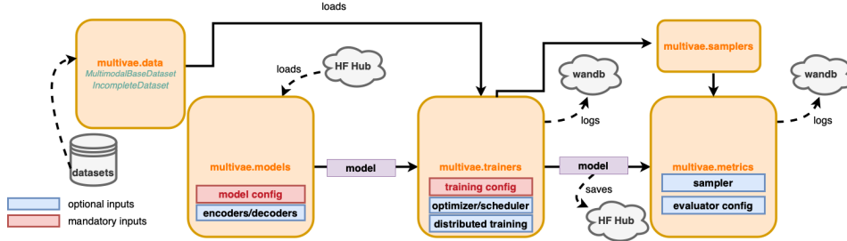
Figure 2: Schematic diagram of the MultiVae library.
