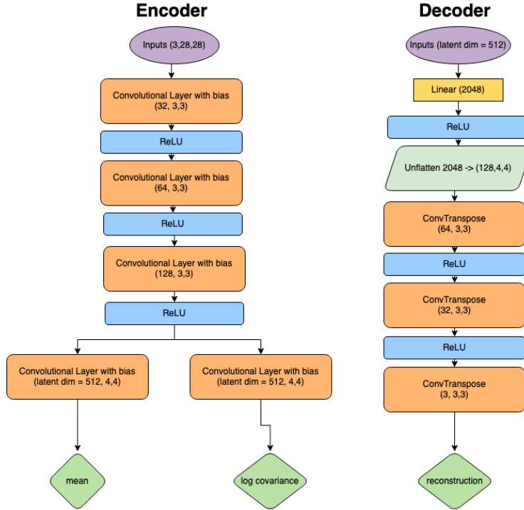
Figure 10: The encoder, decoder architectures used for the comparison between models in section 4.2.
