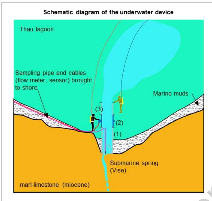
Figure 3. Principle diagram (not to scale) of the instrumentation of the submarine spring in its context of emergence according to the diving explorations. (1): flow collector, (2): flowmeter, (3): stilling tube.
