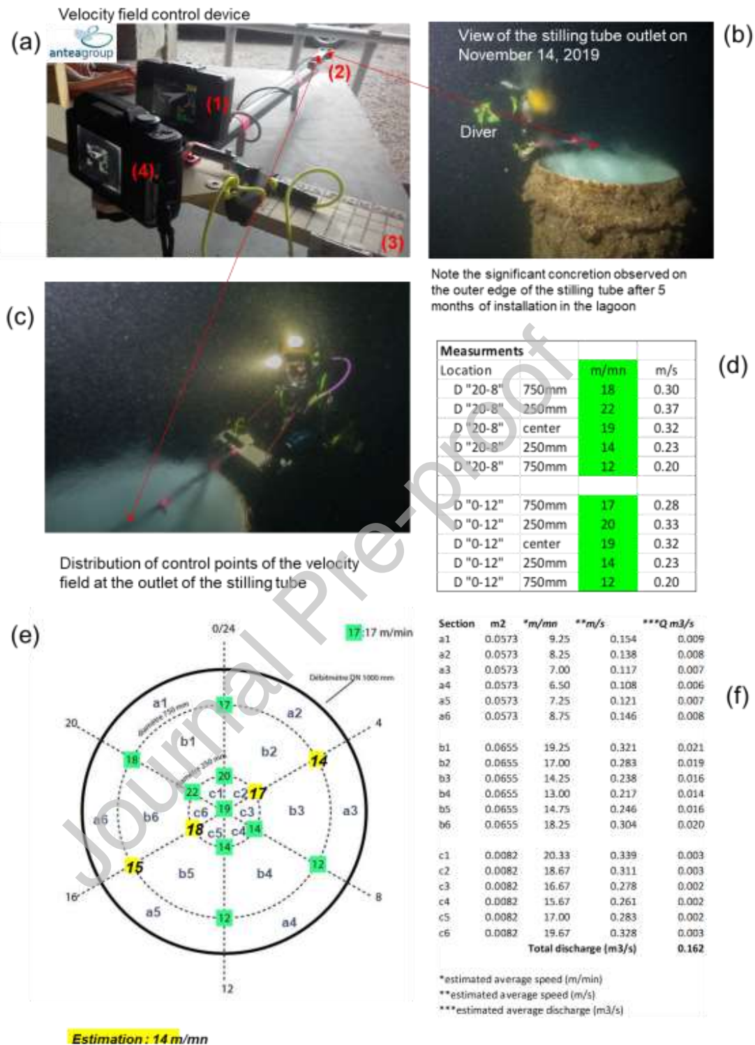
Figure 8. (a) View of the device specially developed to performed punctual velocity controls at the outlet of the stilling tube [1: Seacraft ENC underwater navigation unit, 2: flow velocity sensor, 3: underwater slate, 4: waterproof camera]. (b, c) Diver performing a velocity control
