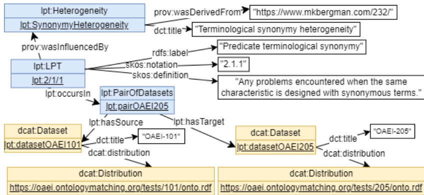
Figure 13. An example of formalization of a LPTs in RDF.
