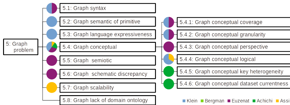
Figure 11. Part of the classification of LPTs: Graph problems.
