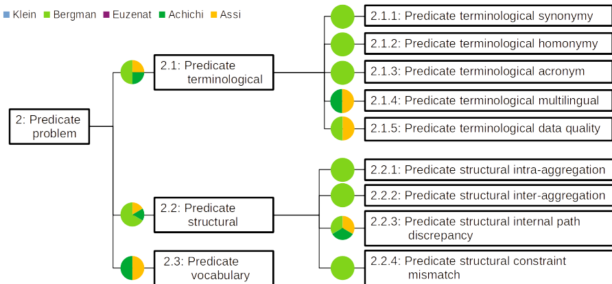
Figure 8. Part of the classification of LPTs: Predicate problems.
