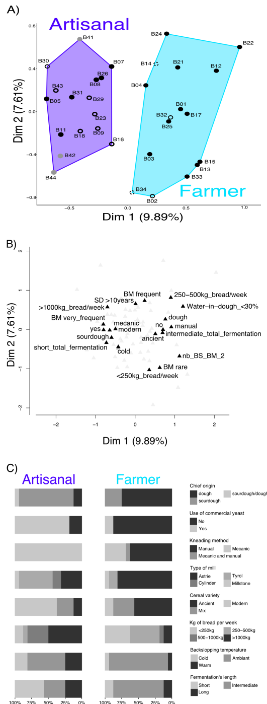
Figure 2: Multiple Correspondence Analysis (MCA) based on 28 categorical variables describing bread making practices. A) Representation of bakers. Each point represents a bakery. The purple area on the left brings together baker with “artisanal” practices and the light blue area on the right the bakers with “farmer” practices. The dot’s colors indicate the PCoA cluster of the sourdough fungal community (see Figure 5). Black dots for group 1, empty dot for group 2, grey for group 3. The fungal community of the sourdough of baker 14 was not studied. B) Representation of the 20 first categories that contributed the most to the MCA axes. The category, which corresponds to a class of a variable, is written next to the
