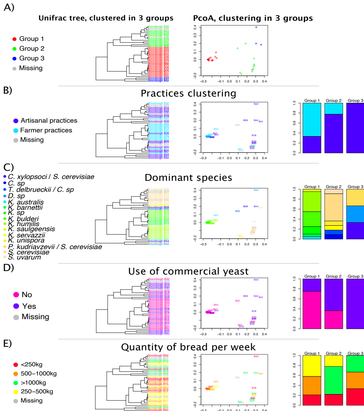
Figure 5: Clustering of sourdough fungal communities based on weighted UniFrac distances and association with baking practices. The weighted UniFrac distance between communities takes into account the relative abundance of the observed species as well as their phylogenetic relationships. In all panels, the clustering of sourdoughs fungal communities based on their UniFrac distances is shown on a tree on the left and on a Principal Component Analysis (PcoA) in the center. Panel A shows the three groups of fungal communities formed based on their weighted UniFrac distances. Panels B through E highlight the distribution of a principal variable in these three groups of fungal communities. The distribution is shown by coloring the different levels of the variable on the tree and on the PcoA but also as a barplot on the right side of the panel. Panel B shows the distribution of the two types of bread making practices, panel C the dominant yeast species, panel D the use of a commercial yeast starter, panel E the amount of bread made each week. Group 1 contains sourdough fungal communities whose dominant species is a Kazachstania species. Group 2 contains sourdough fungal communities whose dominant species is Saccharomyces cerevisiae . Group 3 contains sourdough fungal communities in which two yeast species co-occurred, one being S. cerevisiae . The yeast genus in panel C is abbreviated with, C. for Candida , D. for Dipodascaceae , K. for Kazachstania , S. for Saccharomyces , T. for Torulaspora .
