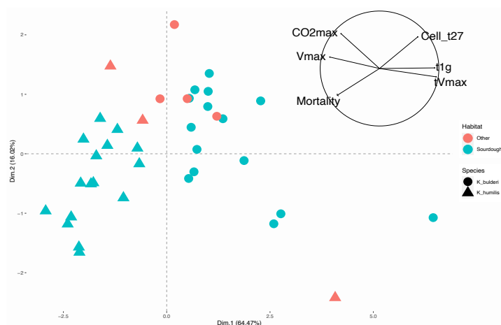
Figure 6: Principal component analysis of 37 K. humilis and K. bulderi strains based on the quantitative variation of maximum CO_2 production ( CO_2max ), fermentation latency phase ( t_{1g} ), maximum CO_2 production rate ( V_{max} ), time to reach the maximum production rate ( tV_{max} ), log of population size and mortality at the end of the fermentation. The correlations between variables are presented on the right while the figure on the left shows the projection of strains on the first two axes representing 70.64% of the variation. The strains are colored according to their habitat of origin. Sourdough strains are indicated in blue and non-sourdough strains in red. Their species is indicated by symbol. Kazachstania humilis strains are indicated by a circle and Kazachstania bulderi strains by a triangle.
