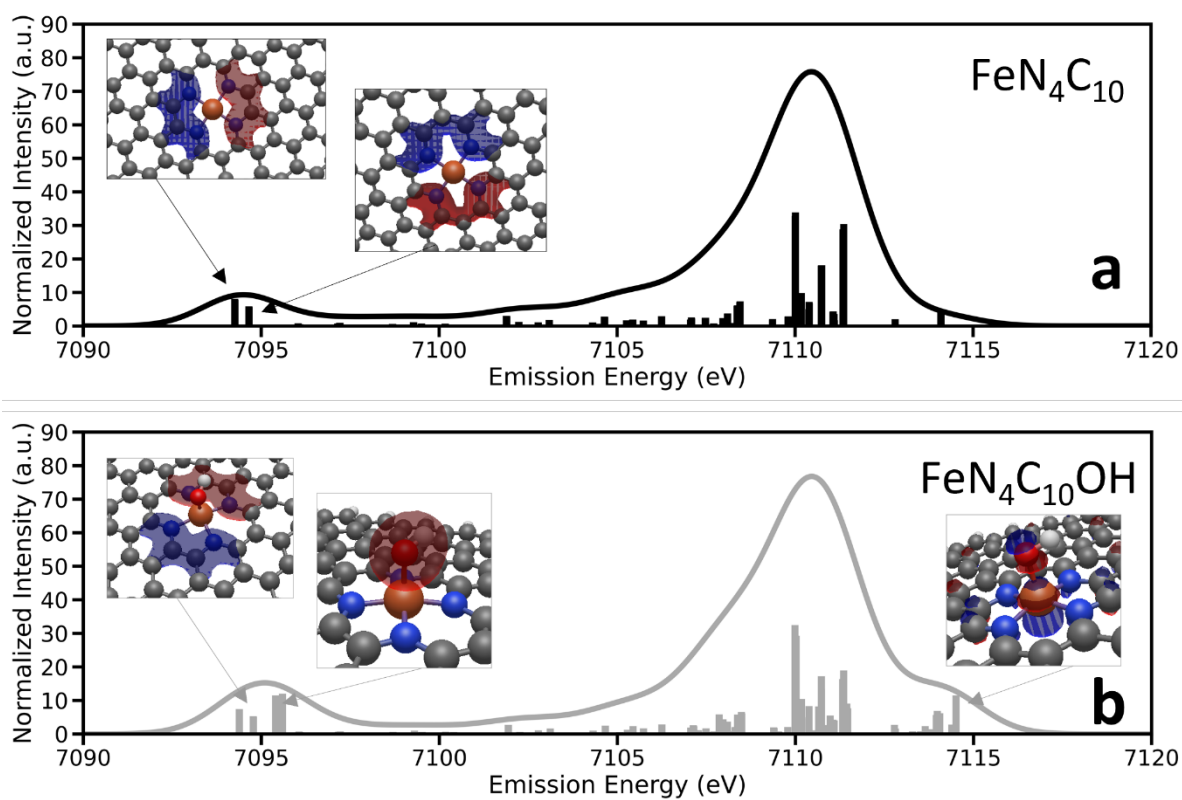
Figure 4. Calculated VtC XES spectra for \text{FeN}_4\text{C}_{10} and \text{FeN}_4\text{C}_{10}\text{OH} sites and representative molecular orbitals giving rise to some of the transitions.
