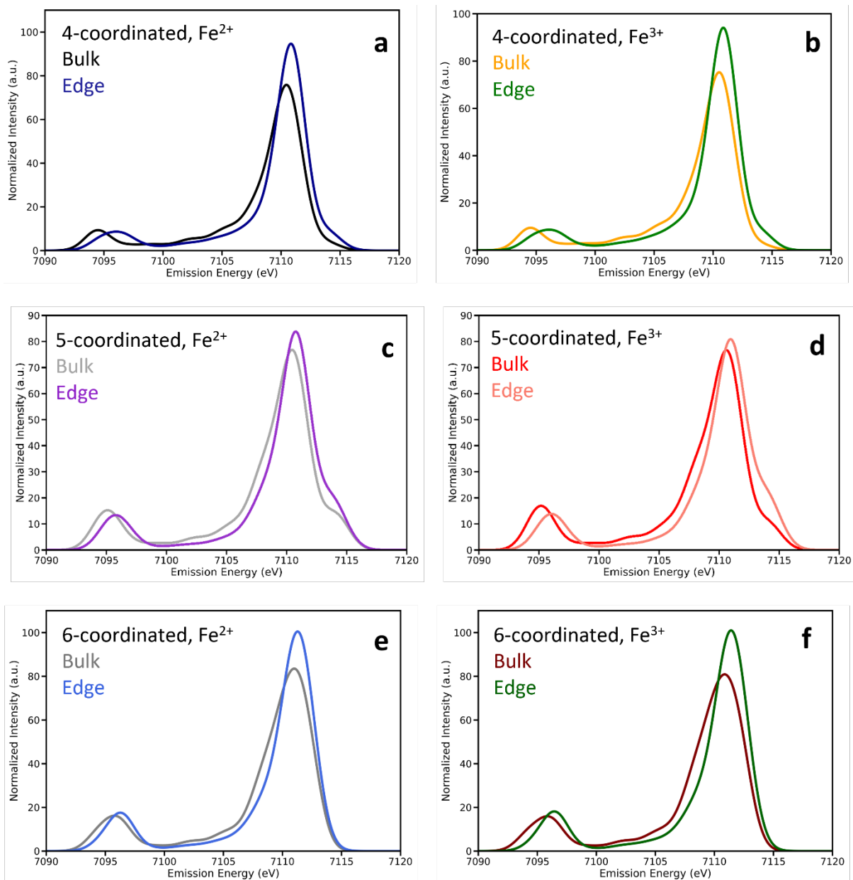
Figure 5. Calculated VtC XES spectra for bulk- and edge-located pyridinic 4-coordinated \text{FeN}_x\text{C}_y (a, b), 5-coordinated \text{FeN}_x\text{C}_y\text{OH} (c, d) and 6-coordinated \text{FeN}_x\text{C}_y(\text{OH})_2 sites (e, f). Two oxidation states of iron atoms \text{Fe}^{2+} (a, c, e) and \text{Fe}^{3+} (b, d, f) are compared.
