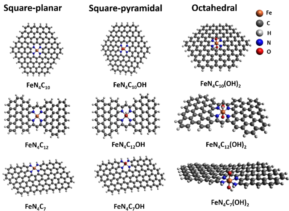
Figure 2. \text{FeN}_x\text{C}_y model structures used in this work.
