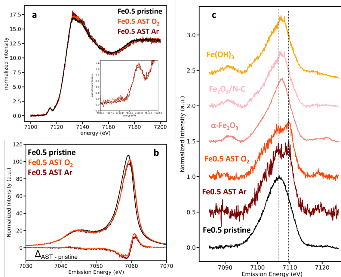
Figure 1. Fe K \beta HERFD XANES (a), K \beta mainline (b) and VtC XES spectra (c) obtained on Fe 0.5 -based electrodes before and after the ASTs. Panel c also contains VtC spectra for bulk and nano-sized Fe 2 O 3 as well as Fe(OH) 3 references. The VtC signals have been vertically shifted for the sake of clarity.
