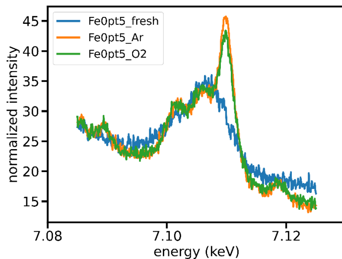
Figure S2. The VtC XES spectra recorded on Fe0.5-based catalyst layers before (fresh) and after the AST tests under Ar and O 2 on the samples presented in Sgarbi et al. [1] The XANES and K \beta XES spectra were presented and discussed in the manuscript mentioned above.
