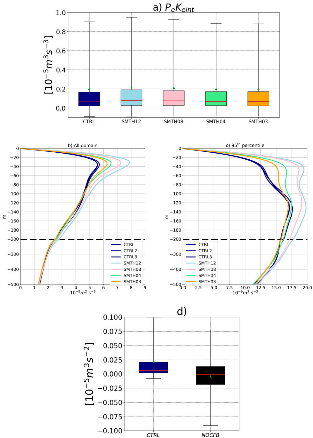
FIG. 6. (a)–(c) As in Fig. 5, but for the baroclinic conversion of energy. (d) Boxplot P_e K_{e_{OA_{ekman}}} from CTRL and NOCFB. TFB causes a reduction of the conversion of potential energy to kinetic energy by baroclinic instability, explaining the damping of the EKE. The TFB-induced Ekman pumping velocities do not cause additional baroclinic conversion of energy.
