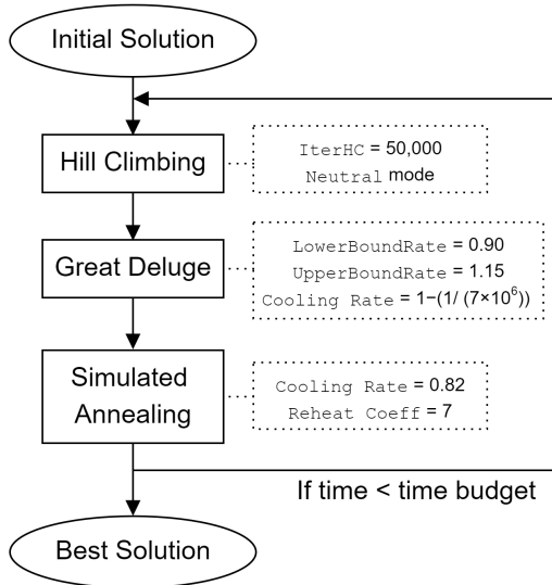
Fig. 2: Composition of HLS method.
