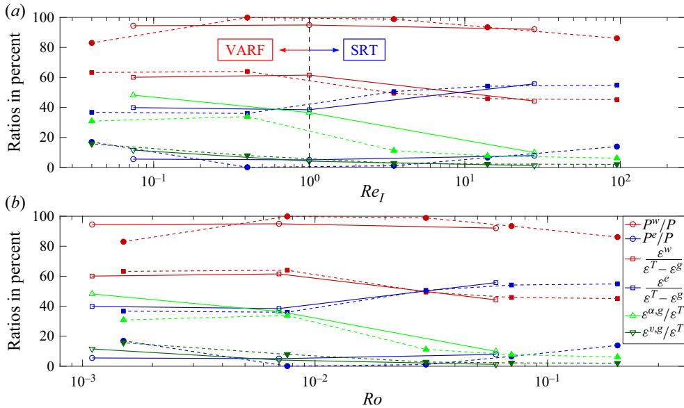
Figure 4. Ratio of forcing P^l/P and ratio of dissipation against the total dissipation without the GM \epsilon^l/(\epsilon^T - \epsilon^g) for waves ( l = w ) and eddies ( l = e ). Ratio of dissipation of the GM due to the added viscosity term on the GM ( \epsilon^{\alpha,g}/\epsilon^T ) and the kinetic dissipation \epsilon^{\nu,g}/\epsilon^T against total dissipation. Results are shown against (a) Re_l , (b) Ro . Open symbols and solid lines are DNS with 512^3 points, filled symbols and dotted lines are DNS with 256^3 points.
