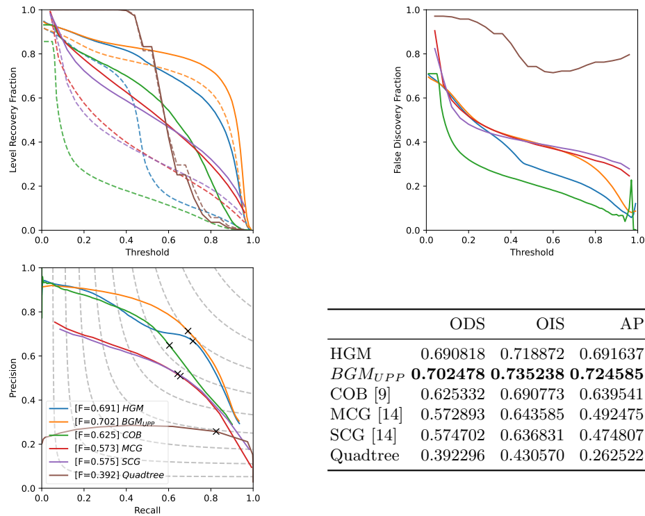
Fig. 5. Benchmarks our methods HGM (blue) and BGM_{UPP} (orange), on COB [9] (green), MCG [14] (red), SCG [14] (purple) and Quadtree (brown) on our ultrametric dataset, with Level Recovery Fraction (top-left), solid lines for high-level, and dashed lines for mid-level), False Discovery Fraction (top-right), Precision-Recall Curves (bottom-left), and quantitative results (bottom-right).
