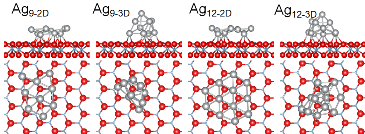
Fig. 7 Side and top views of the \text{Ag}_9 and \text{Ag}_{12} clusters in 2D (1 ML) and 3D configurations. Same color code as in Fig. 5.
