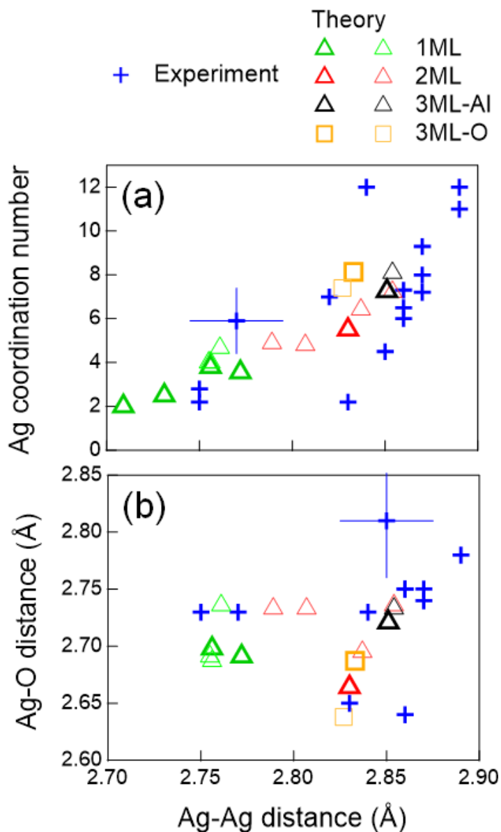
Fig. 4 Comparison between EXAFS measurements (blue crosses) and atomistic simulations related to Ag/ \alpha -Al 2 O 3 (0001) clusters: (a) coordination number of Ag ( CN ) and (b) d_{Ag-O} , as functions of d_{Ag-Ag} . Calculated values, represented by triangles, correspond to different cluster thicknesses: 1 ML (green); 2 ML (red); 3 ML in Al configuration (black) and in O configuration (orange). Bold symbols correspond to the isomers of highest stability. Typical experimental error bars are indicated in each figure.
