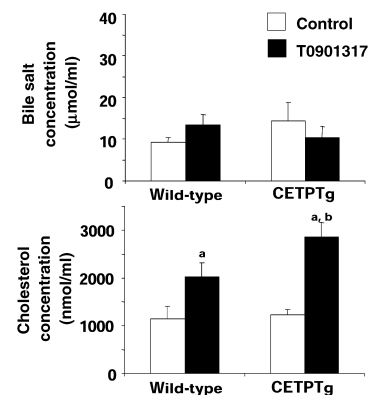
Fig. 4. Cholesterol and bile salt concentrations in the bile of C57Bl6 wild-type and CETPTg mice with or without LXR agonist treatment. Gallbladder bile was collected from C57Bl6 wild-type and CETPTg mice receiving the T0901317 treatment or solvent vehicle only (n = 6 per group). The concentrations of cholesterol and bile acids were subsequently measured as described in Materials and Methods. Values are means ± SEM. a indicates the significance of the difference from homologous mice receiving the solvent vehicle only; b indicates the significance of the difference from C57Bl6 wild-type mice treated with the T0901317 LXR agonist ( P < 0.05 ; Mann-Whitney test).
