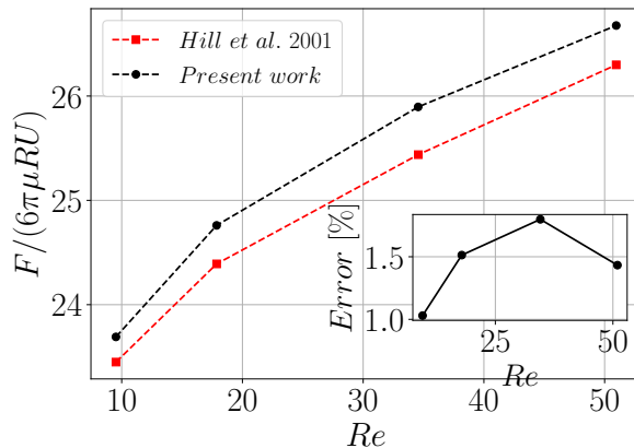
Fig. 4 The non-dimensional drag force on a three-periodic simple cubic array of \varepsilon = 0.592 as a function of Re . The results are compared with the work of Hill et. al Hill et al (2001b) . Inset: the relative error shown as a percentage.
