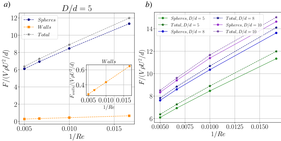
Fig. 13 a) Force contributions on the pressure drop for D/d = 5 , where most of it comes from the spheres. Inset: The force at the walls is enlarged for clarification. b) Total force of the system and total force over the spheres for D/d = 5, 8 and 10 . We observe that for all the cases considered most of the contribution comes from the spheres arrangements and not from the walls themselves.
