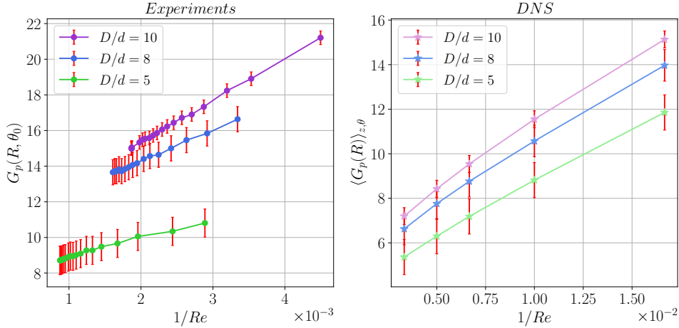
Fig. 11 Non-dimensional pressure gradients G_p = (\Delta p/L)/(\rho U^2/d) as a function of 1/Re . Left: Experimental results, \varepsilon \approx 0.4 . Right: Numerical results, with \varepsilon \approx 0.5 . The error bars for both results correspond to the variability at the walls measured numerically, which increase with the confinement effects.
