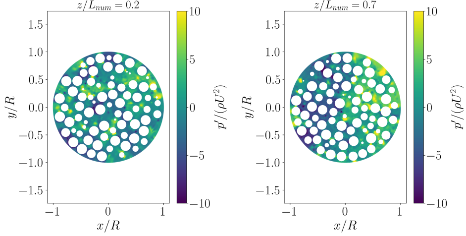
Fig. 6 Pressure field variations p' at two different heights in the bed, for D/d = 10 , \varepsilon = 0.518 and Re = 200 . Results from Direct Numerical Simulations.
