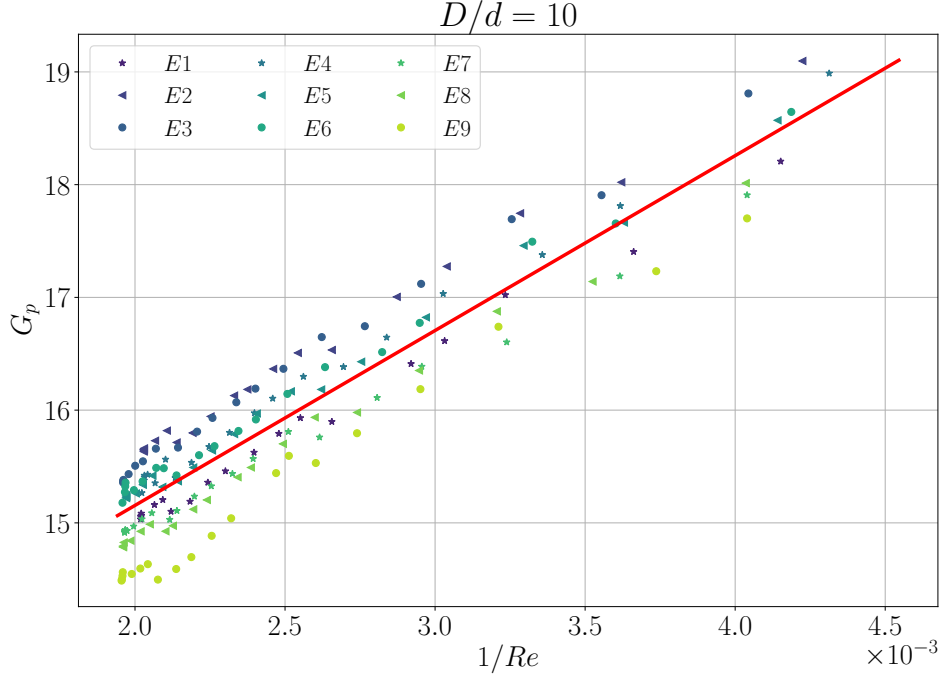
Fig. 7 Pressure drop measured experimentally for nine different random arrangements of spheres with D/d = 10 (shown in different colors and symbols). The red solid line is the average linear fit \overline{G_p} = \overline{\beta} + \overline{\alpha}/Re obtained by averaging the linear fits G_p = \beta + \alpha/Re of the different realizations.
