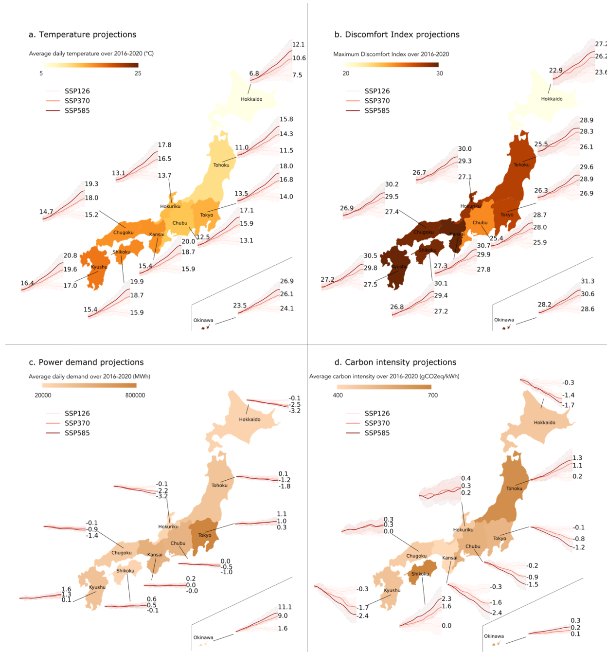
Figure 2: Current and future projections under climate change of average daily temperature (a), DI (b), power demand (c), and carbon intensity (d) for the ten regions of Japan. The color scale on the maps indicates the level for the period 2016-2020. Projections for the period 2020-2100 are shown in solid bands. Lines give mean values from five models;
