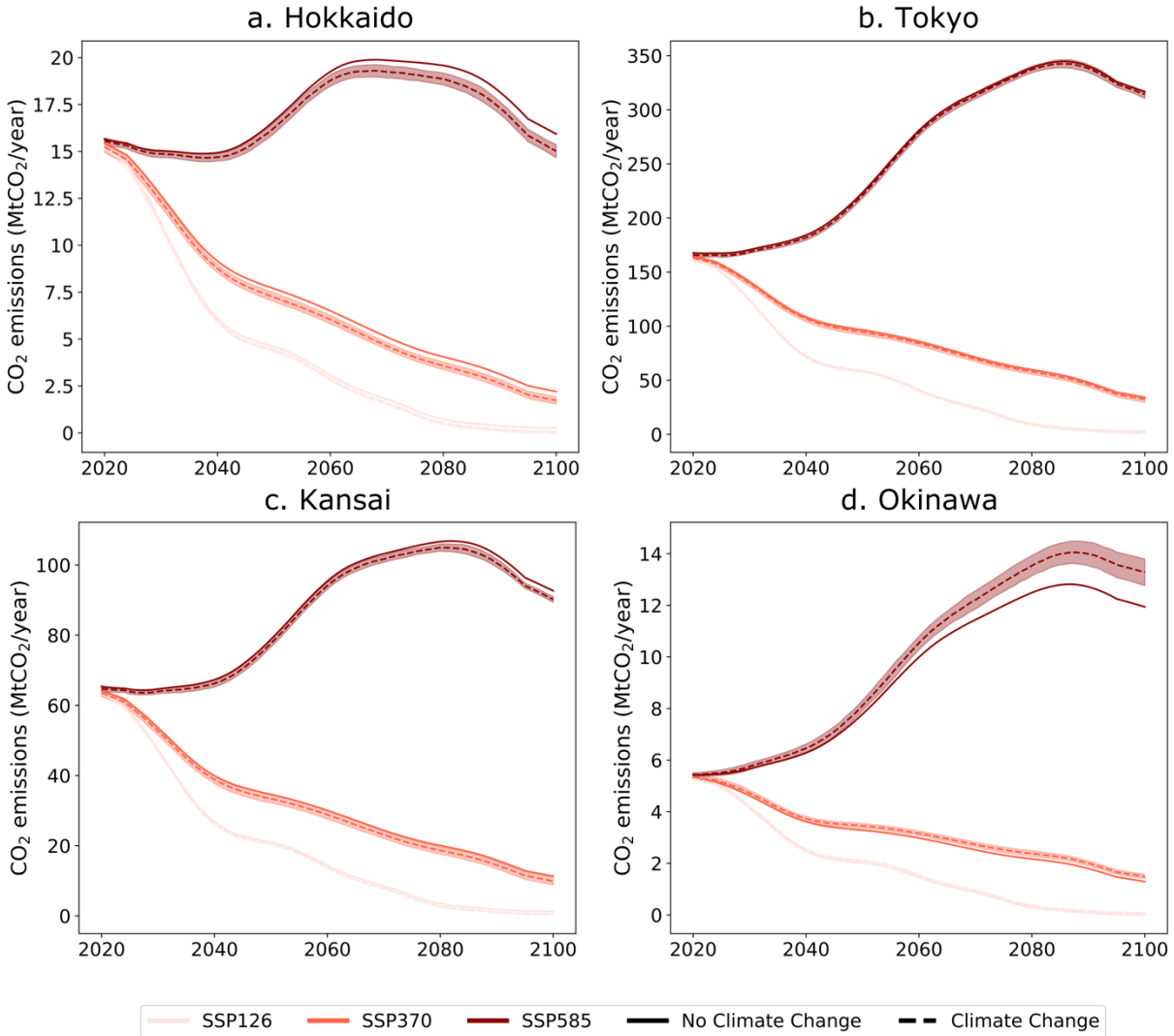
Figure 6: Annual CO 2 emissions from power generation under SSP1-2.6, SSP3-7.0, and SSP5-8.5, after considering socioeconomic impacts with (dashed line) and without (solid line) climate change impact for four regions: Hokkaido (a), Tokyo (b), Kansai (c) and Okinawa (d). The shaded area represents the 1-sigma standard deviation from the five climate models for the scenario considering climate change impact (dashed line).
