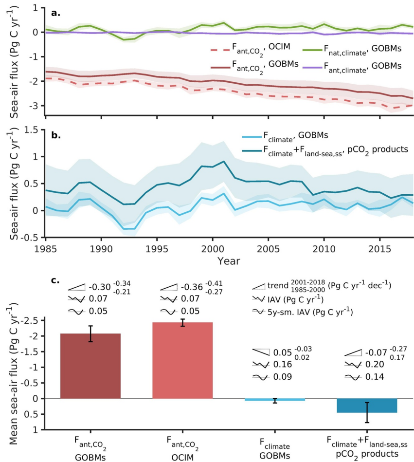
Figure 4. (a) Components of the contemporary net sea-air \text{CO}_2 flux in RECCAP2 global ocean biogeochemical models (GOBMs), using simulations A–D to partition fluxes into the anthropogenic \text{CO}_2 -driven flux ( F_{\text{ant},\text{CO}_2} ), the climate-driven anthropogenic \text{CO}_2 flux ( F_{\text{ant},\text{climate}} ), and the climate-driven natural \text{CO}_2 flux ( F_{\text{nat},\text{climate}} ). Solid curve is the ensemble mean and shading is the ensemble standard deviation. An estimate of F_{\text{ant},\text{CO}_2} from the ocean circulation inverse model (OCIM) is also given by the red dashed curve. (b) The climate-driven sea-air \text{CO}_2 flux ( F_{\text{climate}} ) in the GOBMs, compared with the sum of F_{\text{climate}} and the net land-sea carbon flux ( F_{\text{land-sea,ss}} ) in the \text{pCO}_2 products. Dark curve is the multi-product mean and light shading is the cross-ensemble standard deviation. (c) Summary statistics (as in Figure 2) for F_{\text{ant},\text{CO}_2} from the GOBMs (dark red) and the OCIM (light red), F_{\text{climate}} from the GOBMs (light blue) and F_{\text{climate}} + F_{\text{land-sea,ss}} from the \text{pCO}_2 products (dark blue).
