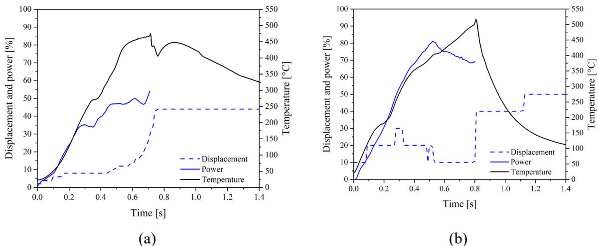
Fig. 1. Temperature monitoring with thermocouples during USW of APC-2 composites with integrated (a) 250 \mu\text{m} PEI for an amplitude of 68 \mu\text{m} , a load of 2.5 bar and a displacement of 30 % (b) 50 \mu\text{m} PEI for an amplitude of 68 \mu\text{m} , a load of 2.5 bar and a time of 0.8 s.
