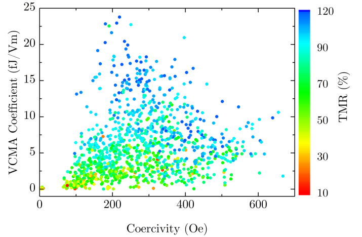
Fig. 7. Dependence of VCMA coefficient with device coercivity and tunneling magneto-resistance.
