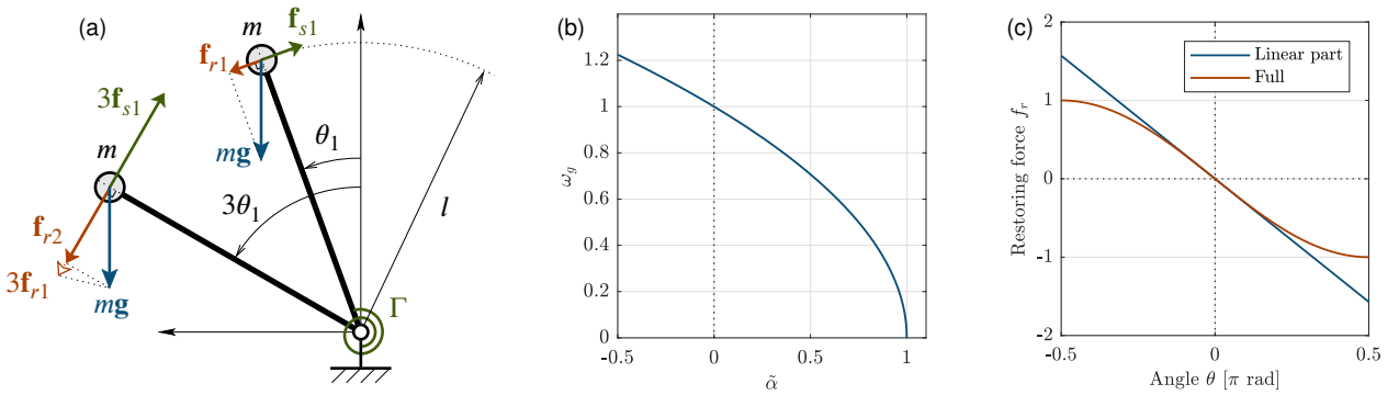
Figure 17: (a) Pendulum shown in two positions along with restoring force \mathbf{f}_r , (b) graph of the natural frequency \omega_\eta of the pendulum as a function of the gravity parameter \tilde{\alpha} (normalized), and (c) graph of the restoring force f_r as a function of angle \theta (normalized).
