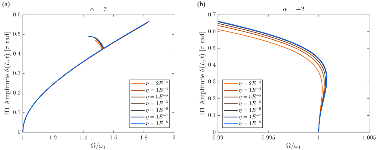
Figure 10: Effect of dimensionless parameters on the first nonlinear mode, isolation of the effect of \eta for \alpha \neq 0 : (a) amplitude of the first harmonic H1 of \theta at the free end of the beam for different values of \eta in the standing configuration ( \alpha = 7 ), (b) the same as (a) but in the hanging configuration ( \alpha = -2 ).
