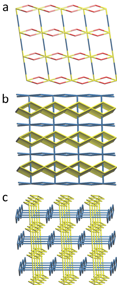
Fig. 5 (a) Nodal representation of the diperiodic network in 4 (yellow, tetranuclear U 4 O 2 nodes; red, kpim 2- edges; blue, bcpmb edges). (b) Nodal representation of the crossing of the two families of layers. (c) Nodal representation of the polycatenated framework.
