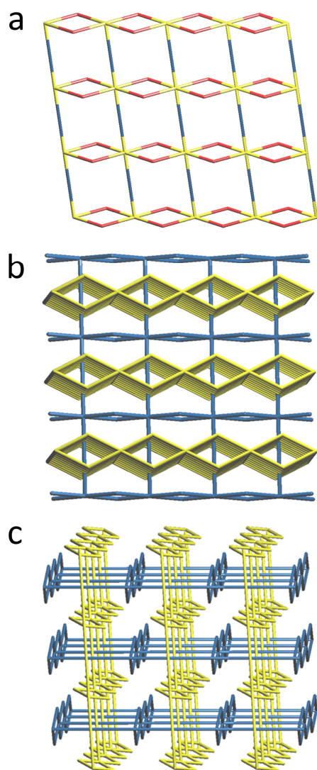
Fig. 5 (a) Nodal representation of the diperiodic network in 4 (yellow, tetranuclear U_4O_2 nodes; red, k_{pim}^{2-} edges; blue, b_{cpmb} edges). (b) Nodal representation of the crossing of the two families of layers. (c) Nodal representation of the polycatenated framework.
