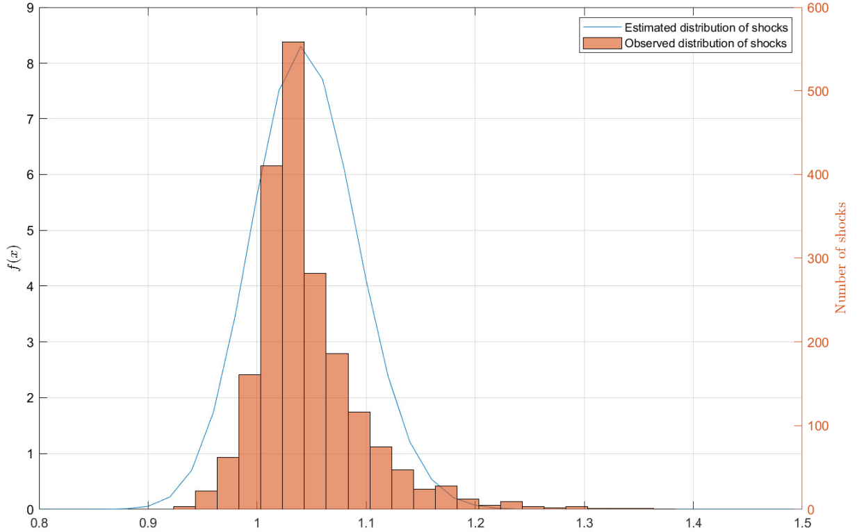
Figure 3: Probability density function of shocks
