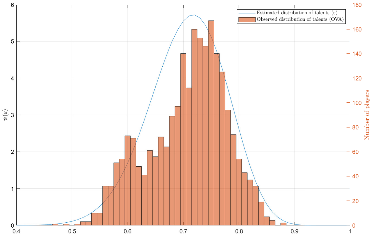
Figure 2: Probability density function of skills
