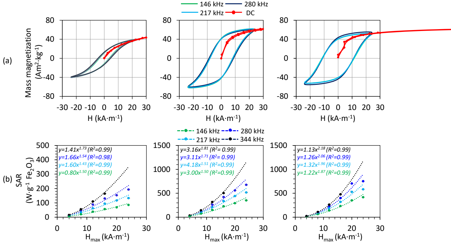
Figure 5. From left to right: Plots of (a) hysteresis loops at f=146, 217 and 280 \text{ kHz} superimposed with the DC curve at low applied H and (b) SAR vs. H_{\text{max}} fitted with a power law of samples NF1, NF4 and NF6 respectively.
