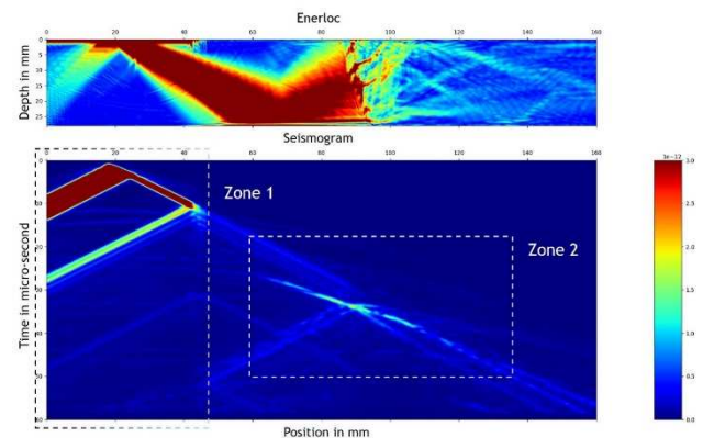
Figure 2. Ultrasonic propagation and seismogram for configuration T60 and position P70 of the emitter. Images voluntarily saturated to enhance propagation through weld
