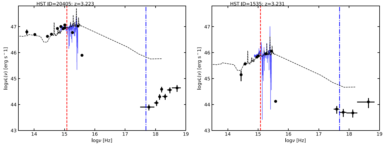
Figure C1. Rest-frame broad-band photometric spectral energy distributions for J2142–4420 ( HST ID = 20405) and J2142–4419 ( HST ID = 1535) from the near-infrared to the X-rays. Data are shown with black points. The MUSE plus HST spectrum for the two quasars is shown with a blue line. We also overplotted the SED for radio-quiet AGN published by Shang et al. (2011) as a reference. The vertical red dashed and blue dot–dashed lines mark the 2500 Å and the 2 keV energies, respectively.
