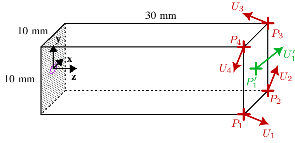
Fig. 4. Conditions for the two case studies, with one target displacement (green) or 4 target displacements (red) with highlighted pneumatic supply (purple) and fixed surface (dashed)
