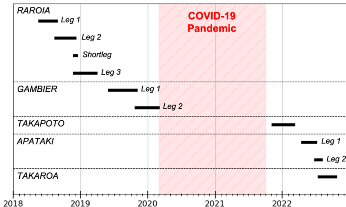
Figure 3: MANA project deployments between May 2018 and November 2022. Gambier Islands are another site studied from mid-2019 to February 2020. It is a group of high islands and data will be presented elsewhere because the sampling strategy obey to different criteria than atolls.
