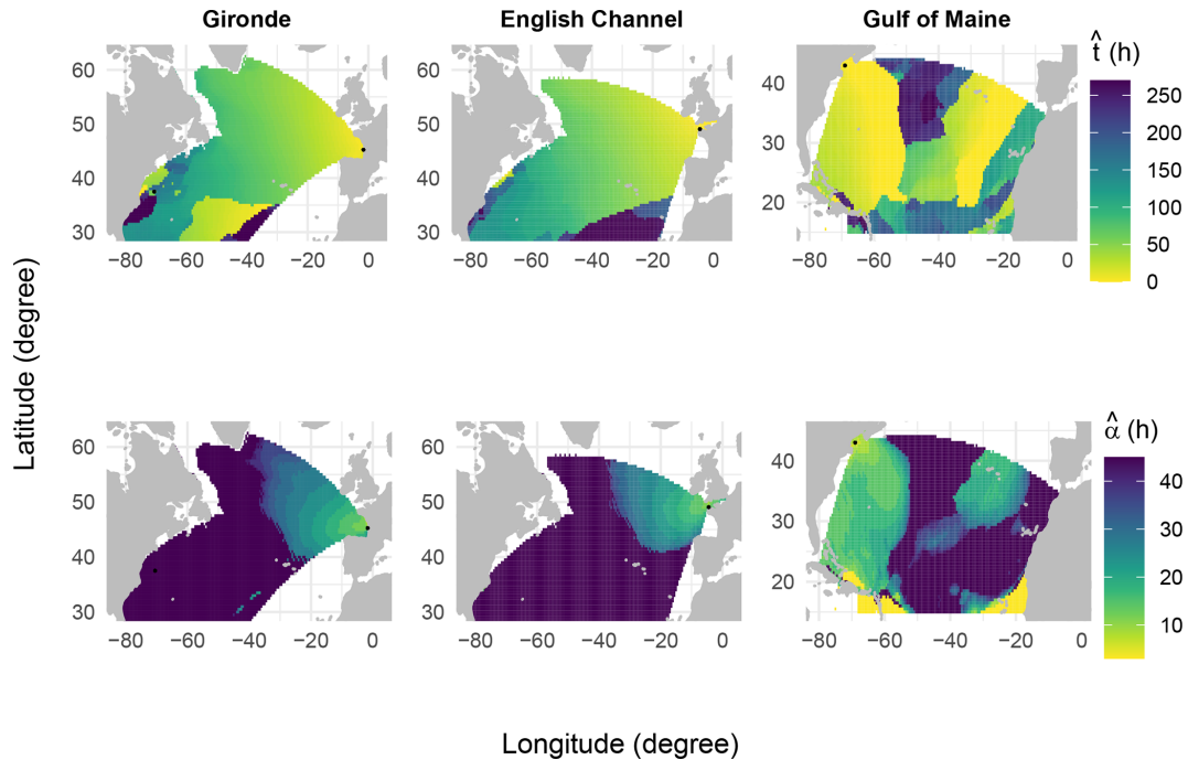
Figure 7. Estimated travel time of waves (top panel) and the temporal width (bottom panel) using Eq. (9) in the three locations.
