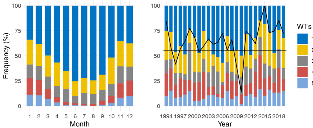
Figure 15. Monthly and annual (in December–January–February) frequency occurrence of WTs in the calibration period. The continuous black line corresponds to the mean annual winter (DJF) time series of the NAO (North Atlantic Oscillation) index, and the horizontal black line indicates when NAO is less or greater than zero. When the continuous black line is below the horizontal line, the NAO is less than zero.
