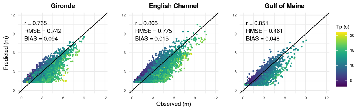
Figure 2. Local model results (Eq. 1) in the validation period at the three considered locations as a function of the peak period ( T_p ).
