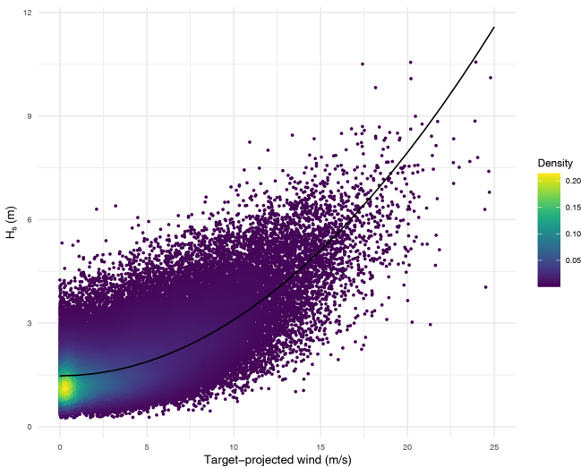
Figure 6. Target-projected wind at point located in (45.5° N, 3.5° W) versus H_s and the estimated curve line using the model H_s = aW^2 + b in Gironde.
