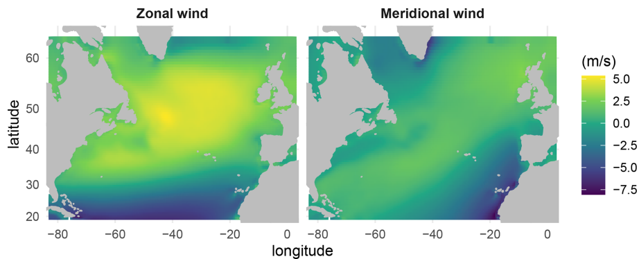
Figure 1. Mean Climate Forecast System Reanalysis (CFSR) zonal and meridional wind components over the period 2014–2019.
