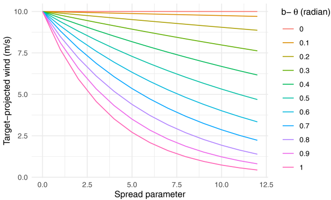
Figure 4. Relationship between the target-projected wind and the spread parameter at varying values of the angle difference b - \theta , with a constant wind speed ( U = 10 \text{ m s}^{-1} ).
