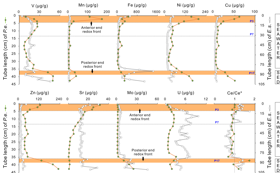
Figure 2. Trace element profiles along chitinous tube of Paraescarpia echinospica (Pe.; green circles); results of Escarpia southwardae (E.s.) are provided for comparison (white squares; Bayon et al., 2020). Ce/Ce^* = 3 \times Ce_N / (2 \times La_N + Pr_N) , where N refers to normalization of concentration against the standard Post-Archaean Australian Shale (PAAS). SED—sediment.
