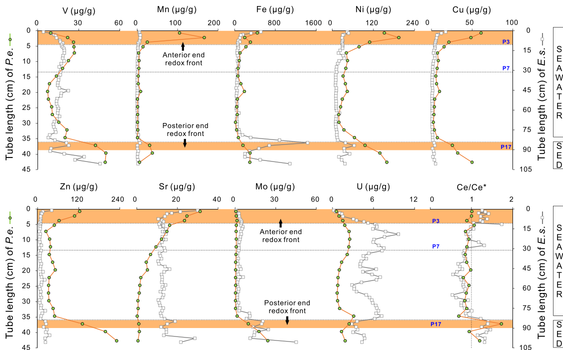
Figure 2. Trace element profiles along chitinous tube of Paraescarpia echinospica ( Pe. ; green circles); results of Escarpia southwardae ( E.s. ) are provided for comparison (white squares; Bayon et al., 2020). Ce/Ce^* = 3 \times Ce_N / (2 \times La_N + Pr_N) , where N refers to normalization of concentration against the standard Post-Archaean Australian Shale (PAAS). SED—sediment.
