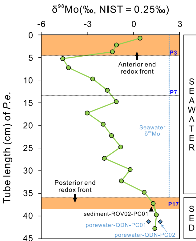
Figure 3. Molybdenum isotope compositions along chitinous tube of Paraescarpia echinospica (Pe.; green circles), average seawater (blue dotted line; Kendall et al., 2017), as well as pore water (blue diamonds) and sediment (black triangle) from study area. NIST—National Institute of Standards and Technology; SED—sediment.
