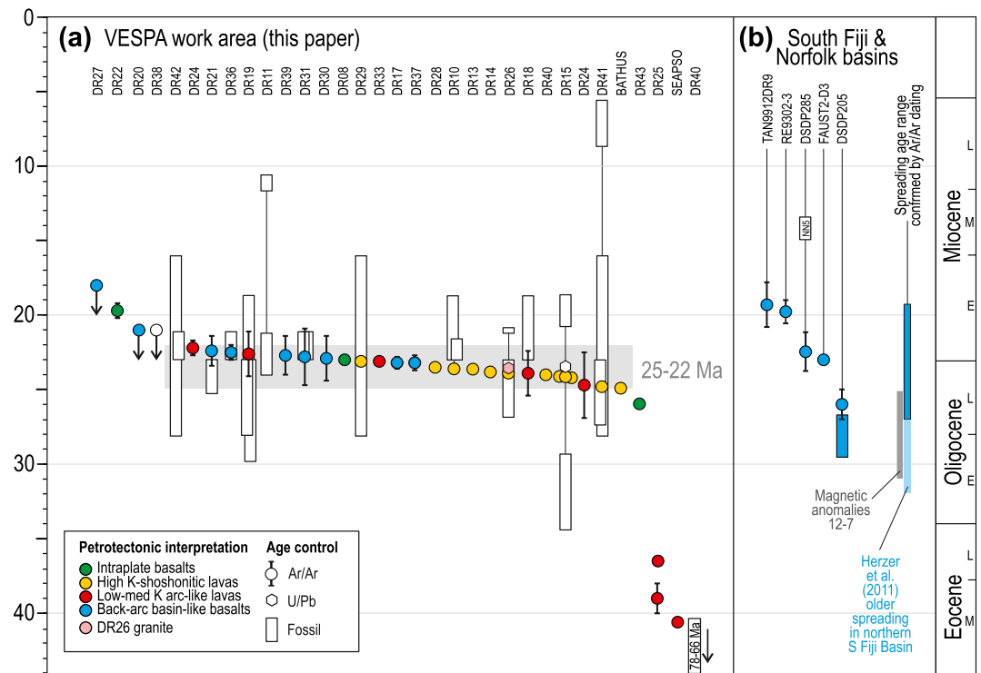
Figure 7. (a) Newly reported ages for VESPA igneous rocks (this paper) ordered left to right from youngest to oldest. Circle and hexagon symbols are Ar/Ar and U/Pb ages, white rectangles are supporting microfossil ages on samples from the same dredge. (b) Previously established direct dating of South Fiji and Norfolk basin crust (Bernardel et al., 2002; Edwards, 1973; Mortimer et al., 1998, 2007, 2014). These, and the VESPA ages, confirm a younger spreading age range than that based on magnetic anomalies (Davey, 1982; Malahoff et al., 1982; Sdrolias et al., 2003; Watts et al., 1977). In both panels, where circles have no error bars, the 2\sigma age error lies within the size of the symbol.
