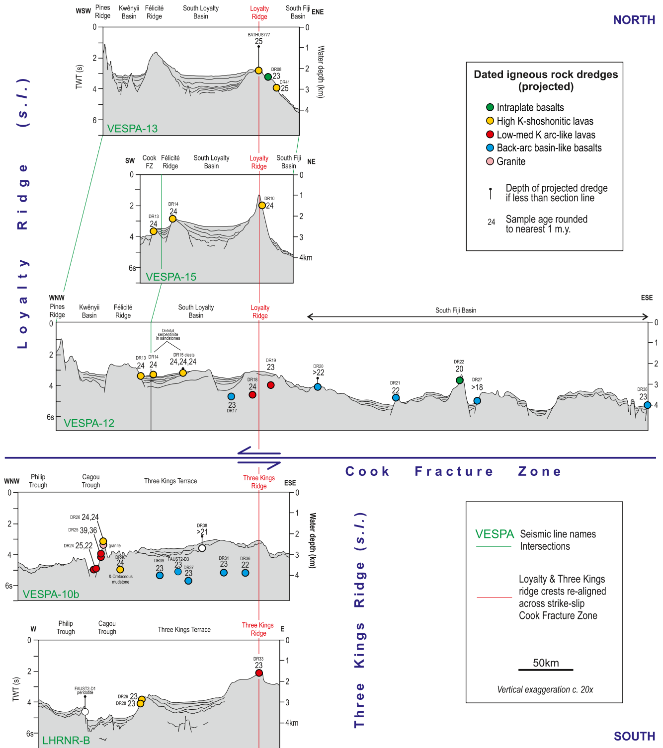
Figure 9. Age and compositional data for VESPA igneous rocks plotted on five lightly interpreted seismic reflection profiles (Mortimer & Patriat, 2016). See Figure 2a for profile locations. Profiles are ordered from north (top of page) to south (bottom of page) and have been positioned left-to right so that the crests of the Loyalty Ridge ( sensu stricto ) and Three Kings Ridge ( sensu stricto ) coincide. Such a restoration of the c. 250 km sinistral offset on the Cook Fracture Zone better shows the relative positions of the Loyalty and Three Kings Ridge VESPA dredge sites. Line LHRNR-B is from Ramsay et al. (1997). TWT = two-way travel time. Patriat et al. (2018) gave interpretations of VESPA seismic lines north of these.
