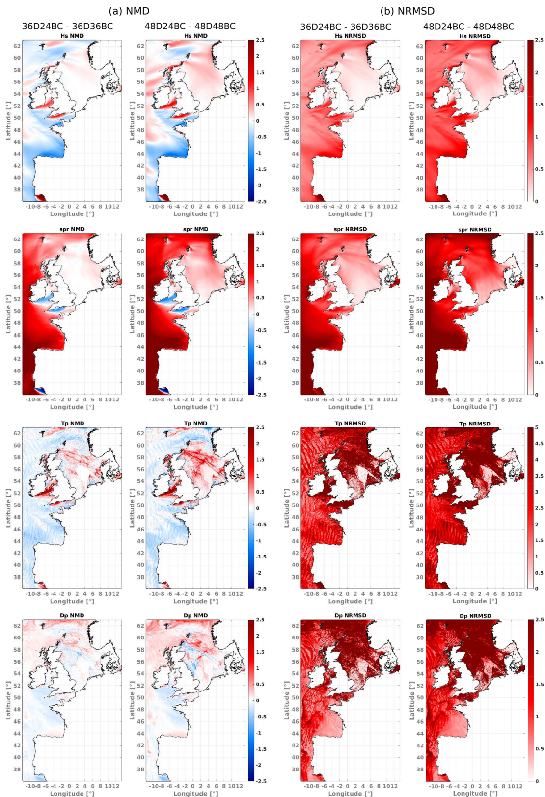
Figure 12. (a) Normalized mean differences (NMDs) and (b) normalized root mean squared differences (NRMSDs) between tests 36D24BC – 36D36BC and 48D24BC – 48D48BC. Analyzed period: February 2011. Color bars represent changes in quantities between tests in percent.
