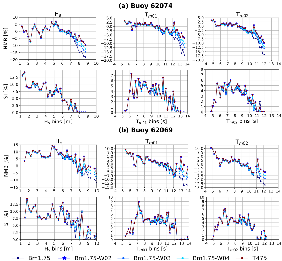
Figure 6. Bias (NMB) and scatter index (SI) for tests leading to T475 (Table 2). Results for January 2014. In (a) and (b) modeled results are compared with buoys 62074 and 62069, respectively. H_s bin size is 0.25 m; periods bin size is 0.2 s. T_{m01} and T_{m02} are computed integrating the spectra in the frequency range 0.0339–0.537 Hz.
