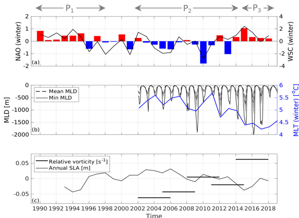
Fig. 5 Temporal variability of the North Atlantic subpolar gyre properties. a Winter North Atlantic Oscillation (NAO) index anomalies from 1990 to 2018, and winter Wind Stress Curl (WSC; N\ m^{-2} ) from 1990 to 2018 (black curve) in the Irminger Sea. b Monthly Mixed Layer Depth (MLD; black curve) and Mixed Layer Temperature (MLT; ^{\circ}C , blue curve) averaged in the Irminger Sea region from 2002 to 2018 computed from ISAS. The uncertainty in the mean MLD is computed as one standard deviation around the mean value. c The black curve represents the annual Sea Level Anomalies (SLA), detrended and offset by its mean (2.7 cm). The horizontal lines show the anomaly of the relative vorticity at 1000 m and average over 4-years periods. The three periods ( P_1 , P_2 , and P_3 ) discussed throughout the manuscript are indicated with arrows on top of the figure.
