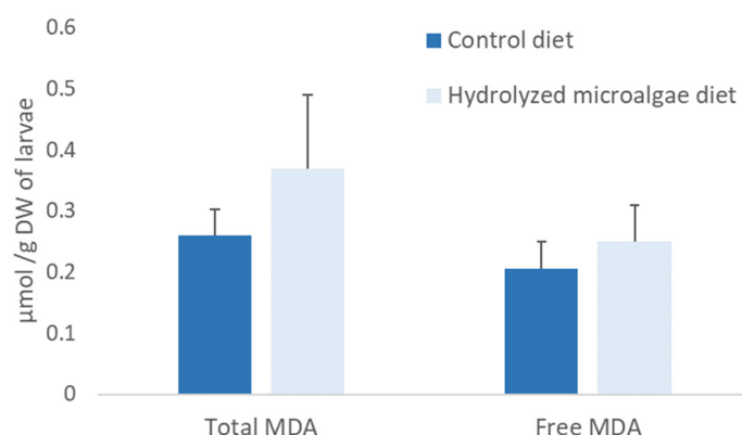
Figure 8. Total and free MDA of sea bass larvae fed control, and hydrolyzed microalgae diets from day 20 to 41 after hatching.
