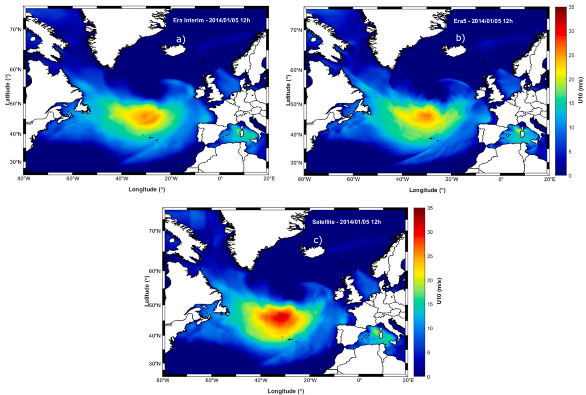
Fig. 8. U_{10} scalar fields in the North Atlantic area for the 5 th of January 2014 at 12h, from ERA-Interim (a), ERA5 (b) and Scatterometer (c).
