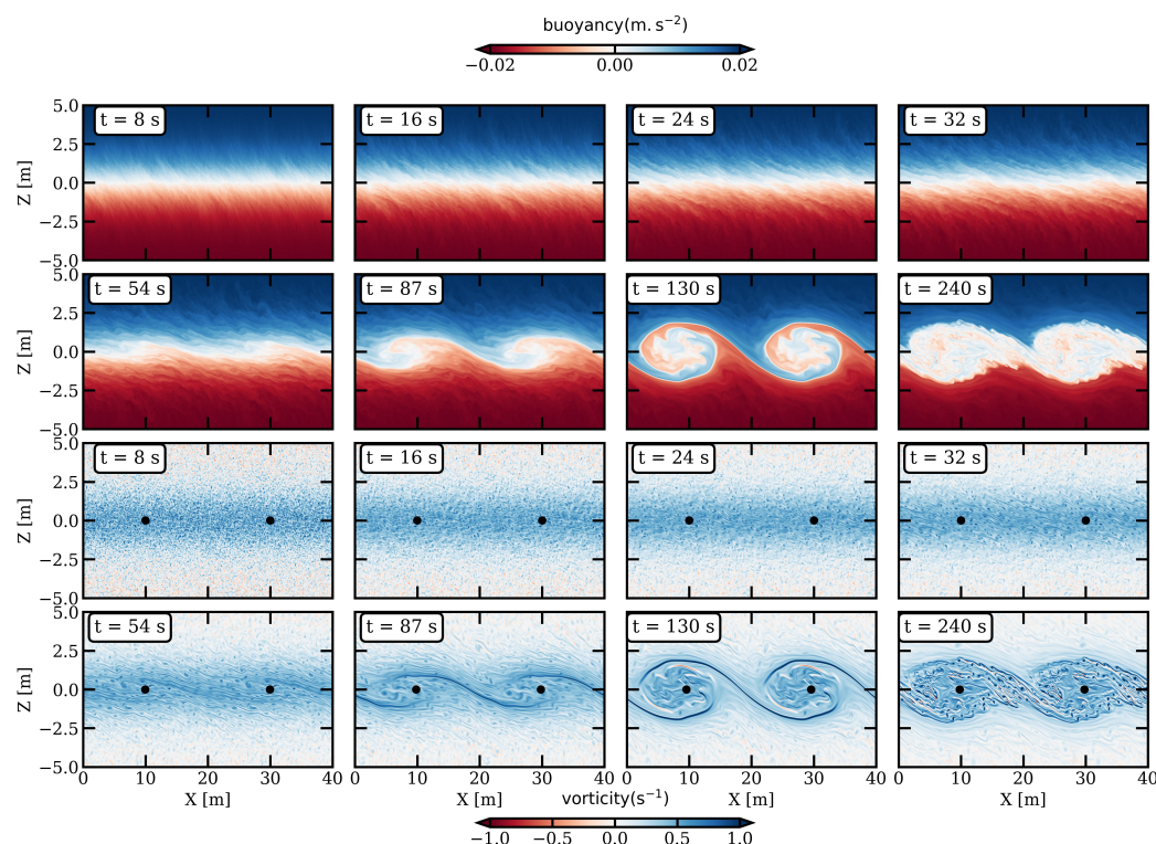
Figure 2. Snapshots from the reference experiment of: buoyancy field ( top two rows ), vorticity field ( bottom two rows ). The black dots in the vorticity field indicate the vorticity centroid of each billow.
