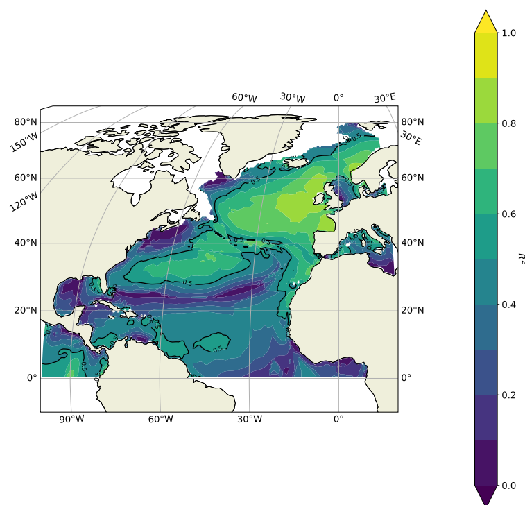
Figure 8. Coefficient of determination ( R^2 ) of all climate modes (i.e., NAO, EA, SCA, EA/WR, PNA, TNH, ENSO, SAM and WEPA) significantly correlated with JFM H_s (see Figure 7). Values close to 1 (to 0) indicate that the JFM H_s variance is well (poorly) explained by the sum of the studied climate modes. The black contour line shows where the 0.5 contour is.
