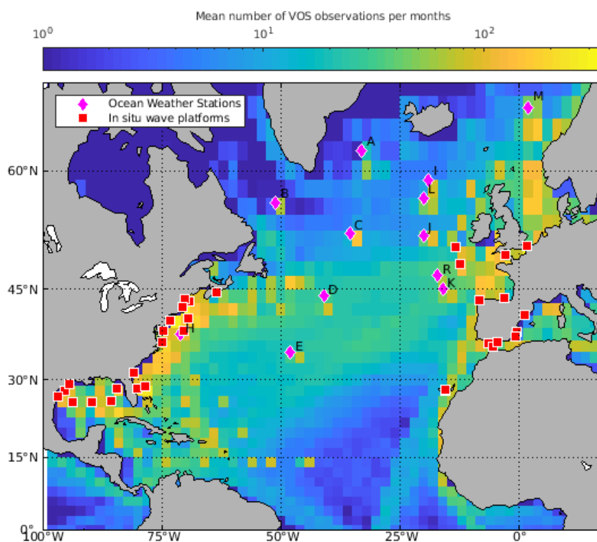
Figure 1. Map of historical (>25 years) wave measurements in the North Atlantic.
