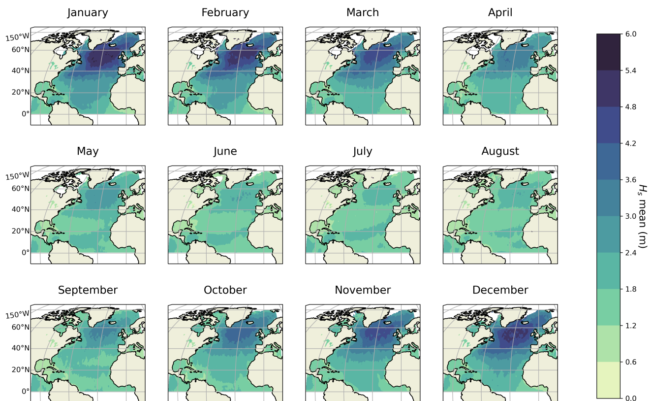
Figure 4. Maps of monthly mean of H_s (m) calculated over the period 1993–2018 using altimeter data.
