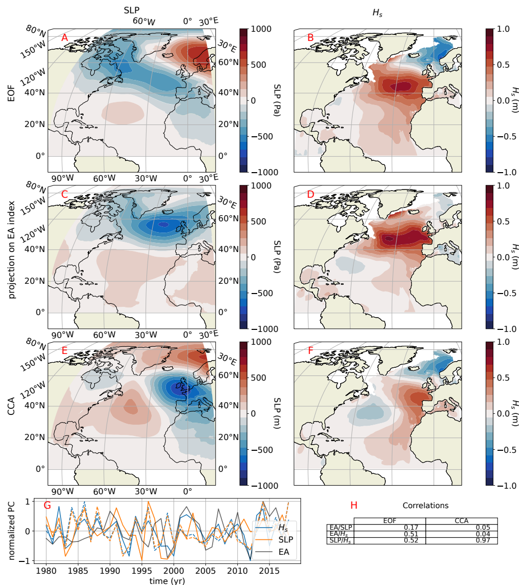
Figure 3. Same as Figure 2 but with the second EOF of SLP (panel (A)) and H_s (panel (B)), projection on the EA index (panel (C,D)) and second CCA mode (panel (E,F)). The explained variability of the second EOF of SLP and H_s is respectively 12% and 24%. The optimized correlation of the H_s and SLP CCA mode is 0.97. Panel (G): normalized PC of SLP (EOF: orange line, CCA dashed orange line) and H_s (EOF: blue line, CCA, dashed blue). The JFM averaged EA NOAA index is shown by a black line. Panel (H): table showing the correlation of the NOAA EA index and the SLP PC (first row), H_s PC (second row) and the correlation of the SLP and H_s PC (third row) for the EOF analysis (first column) and the CCA analysis (second column).
