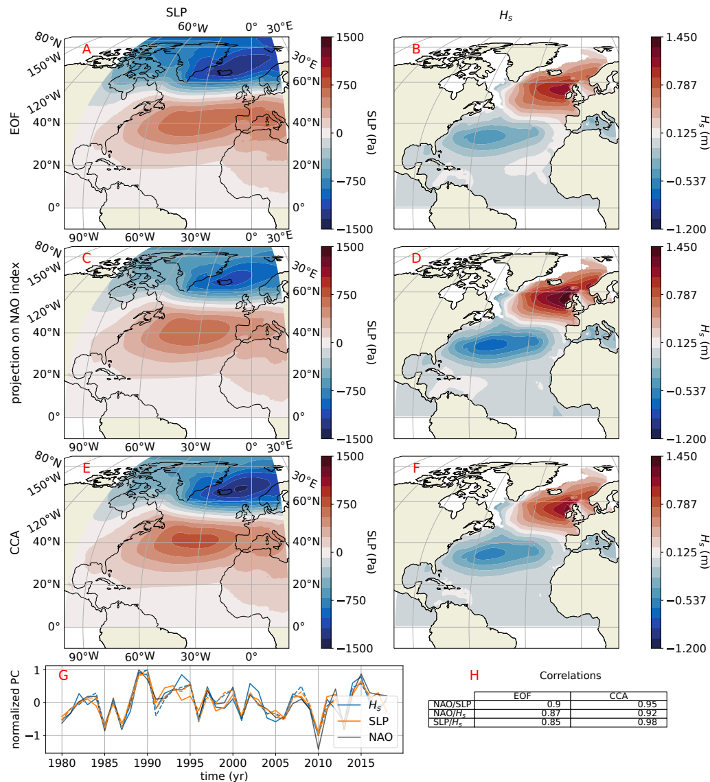
Figure 2. Leading EOF mode of JFM average SLP (panel (A), in Pa) and of JFM average H s (panel (B), in m) calculated with ERA-5 data for the period 1980–2018. Both EOFs are normalized with their respective PC maximum values. The explained variability of the first EOF of SLP and H s are respectively 57% and 41%. Projection of JFM average SLP (panel (C)) and H s (panel (D)) on the JFM average of NOAA NAO index. Leading CCA mode with the corresponding pattern for SLP (panel (E)) and H s (panel (F)). Panel (G): normalized PC of SLP (EOF: orange line, CCA dashed orange line) and H s (EOF: blue line, CCA, dashed blue). The optimized correlation of the H s and SLP CCA mode is 0.98. The JFM averaged NAO NOAA index is shown by a black line. Panel (H): table showing the correlation of the NOAA NAO index and the SLP PC (first row), H s PC (second row) and the correlation of the SLP and H s PC (third row) for the EOF analysis (first column) and the CCA analysis (second column).
