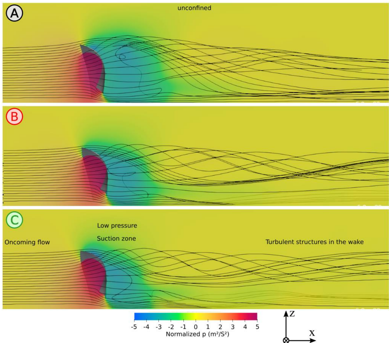
Figure 14: Normalized pressure for different spinnaker trimming using a pressure outlet condition on the top domain plane (OpenFOAM URANSE – k- \omega SST).
