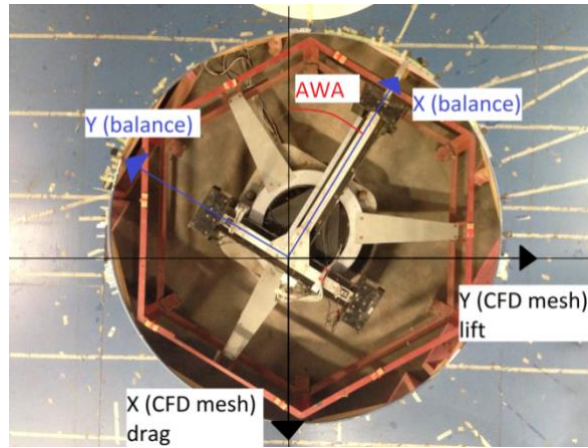
Figure 3: Bird eye's view on the force balance. The hexagonal support frame rotates the force balance to modify the apparent wind angle. (a) is taken when the balance x axis is aligned with the incoming flow (Aubin, 2017).
