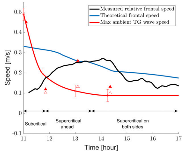
FIG. 7. The plot compares the measured v_{f,obs} (black) and steady-state theoretical v_f (blue) frontal velocities, and demonstrates that several regime transitions (approximately indicated by bottom arrows) occur in relation to IGW front speed criticality. IGW speed ahead of the plume c_a is shown in red circles at 1100 CDT, and per period 1–3 (1100–1230, 1230–1330, 1330–1500 CDT, respectively). Crosses denote c_a uncertainty estimates. The red curve is obtained by spline interpolation from the red circles, and by uniform forward extrapolation after 1500 CDT. Solid (hollow) triangles denote nonlinear (linear) IGW speed in the ambient under the plume, c_{nl} ( c_u ). Triangles symbols relate to the same times as circles but are horizontally offset for visual clarity. Further details on calculations are given in section 4 and in appendixes B–D. Error estimates for c_u and c_{nl} are given in Table E1. The annotations “subcritical,” “supercritical ahead,” and “supercritical on both sides,” refer to F_a < 1 , ( F_a > 1 while F_u \leq 1 ), and both > 1 , respectively.
