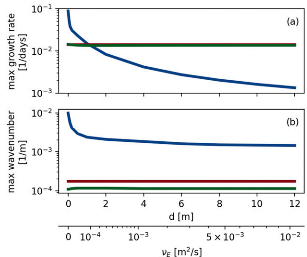
FIG. 5. (a) Growth rate and (b) wavenumber of the fastest growing perturbation as a function of the Ekman layer thickness d or, equivalently, of the vertical diffusivity \nu_E = d^2 f_0 / 2 . Colors as in Fig. 4. The green and red curves in (a) are almost indistinguishable.
