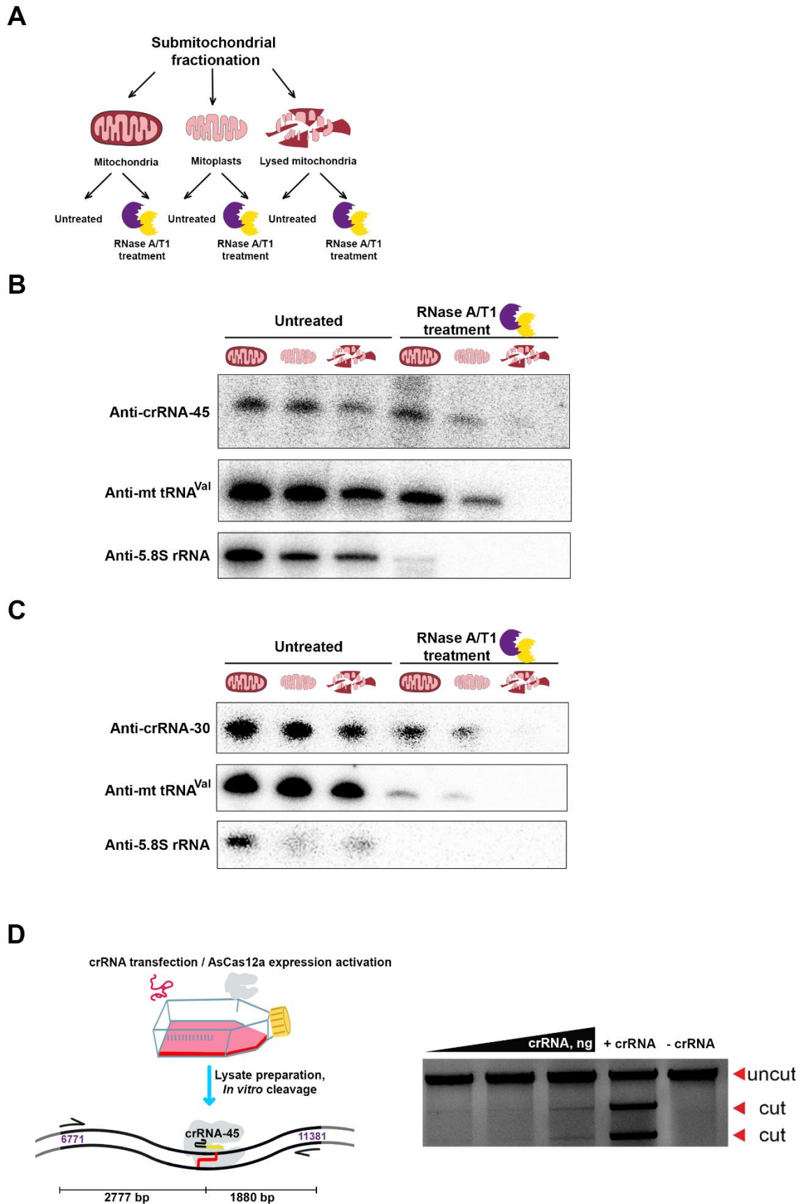
Fig. 6. Submitochondrial localization of AsCas12a crRNAs.
