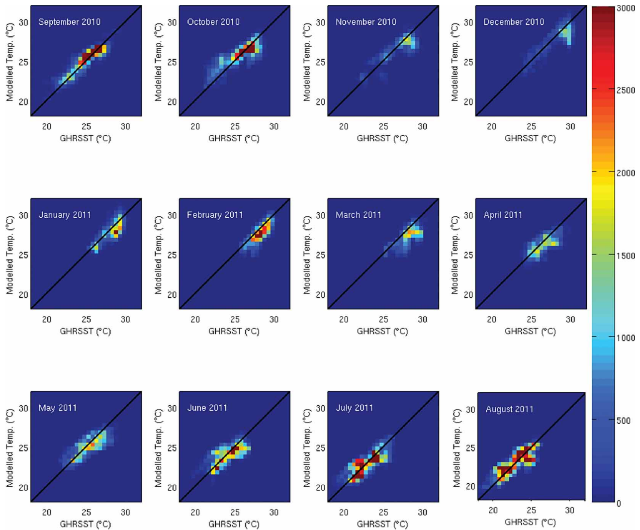
Figure 6. High resolution model to data monthly comparison for the Great Barrier Reef. Two-dimensional histogram of binned GHRSSST data vs. model SST output during the period September 2010 - August 2011. Color denotes the number of observations (frequency) of a particular data/model combination. Dark red denotes the highest mass. The black line denotes the 1:1 relationship between the GHRSSST data and model output. This analysis gives more insight than a typical scatter plot.
