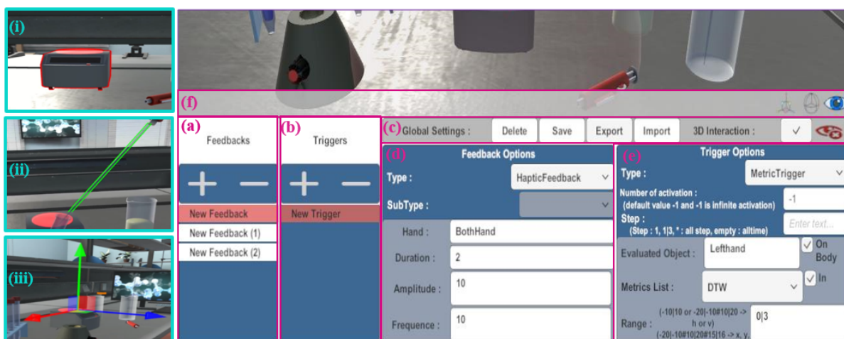
Figure 2: Human Computer Interface (HCI) of GEFEED.
