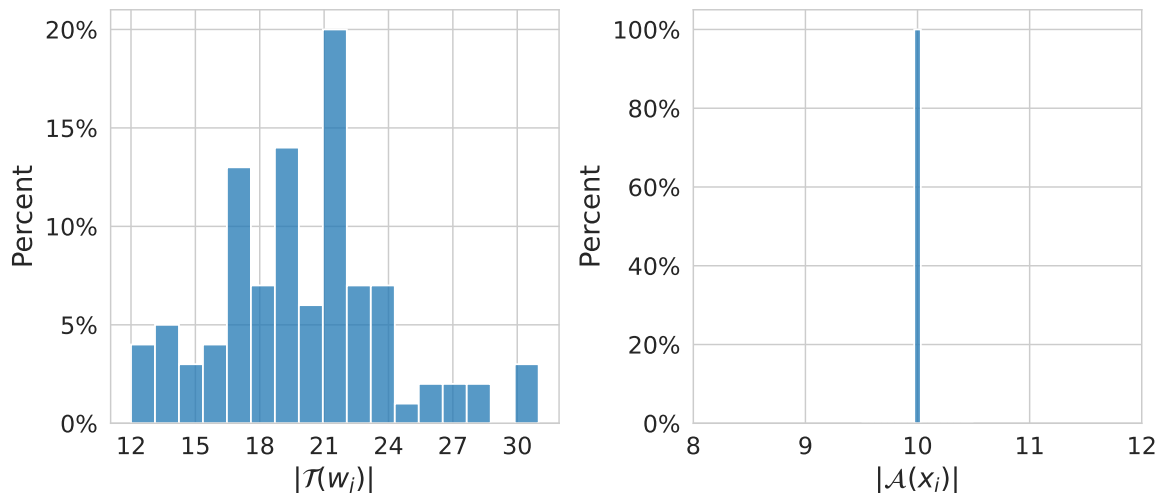
Figure 12: Distribution of number of tasks given per worker (left) and number of labels per task (right) in the setting with simulated discrete difficulty levels.
