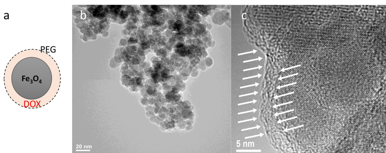
Figure 7. Morphology of doxorubicin-iron oxide nanoparticles: (a) core-shell schematic representation of doxorubicin-loaded iron oxide nanoparticles conjugated with polyethylene glycol with 6000 Da molecular weight, (b) transmission electron microscopy image illustrating the round-shape morphology of the iron oxide nanoparticles, (c) detailed high resolution transmission electron microscopy image of the PEG shell (white arrows).
