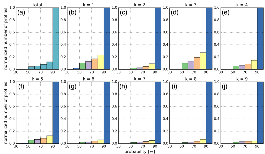
Figure 4. Histograms of the percent posterior probability associated with (a) the full Argo data set and (b–j) each of the nine clusters ( k ) presented in Figure 2. The number of profiles for each 10% bin is normalized by the total number of profiles in the 90–100% bin and are color coded in panels (b)–(j).
