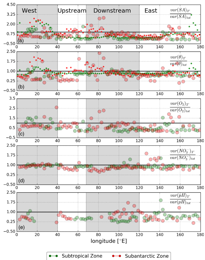
Figure 13. Regional variability of the ratio of binned ( 2^\circ in longitude) over the total variance of (a) absolute salinity (SA), (b) potential temperature ( \theta ), (c) oxygen ( O_2 ), (d) nitrate ( NO_3^- ), and (e) pH, along \sigma_0 , computed across the density classes around the Antarctic Intermediate Water. Markers are color coded as in Figure 12.
