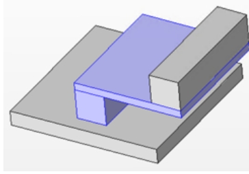
Figure 8: UC with micro-resonator: acrylic part (blue) and steel part (grey).
