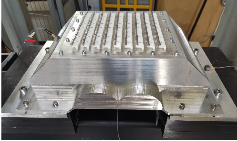
Figure 19: Aluminium GBH mock-up bolted to the experimental stand, with LRM solution applied on the top plate.
