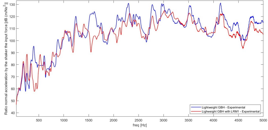
Figure 20: Normalized acceleration at the center of the top plate - Experimental.
