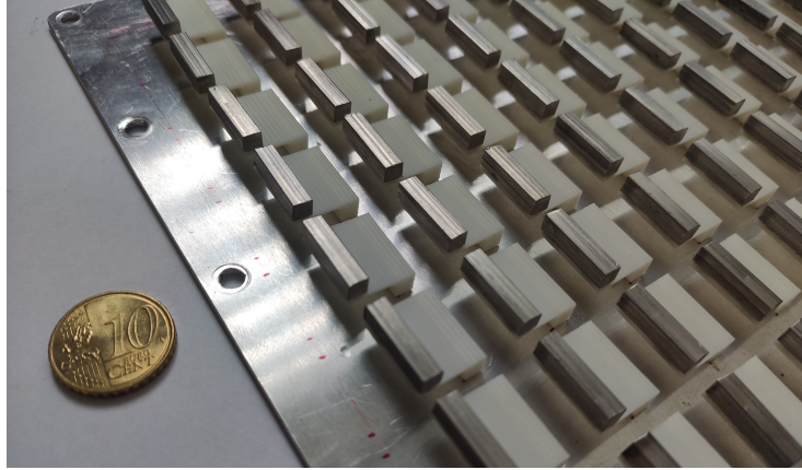
Figure 18: Close-up view of the LRM Plate (aluminium plate with 72 ABS-Steel micro-resonators) next to a 10 cent euro coin (for scale perception).
