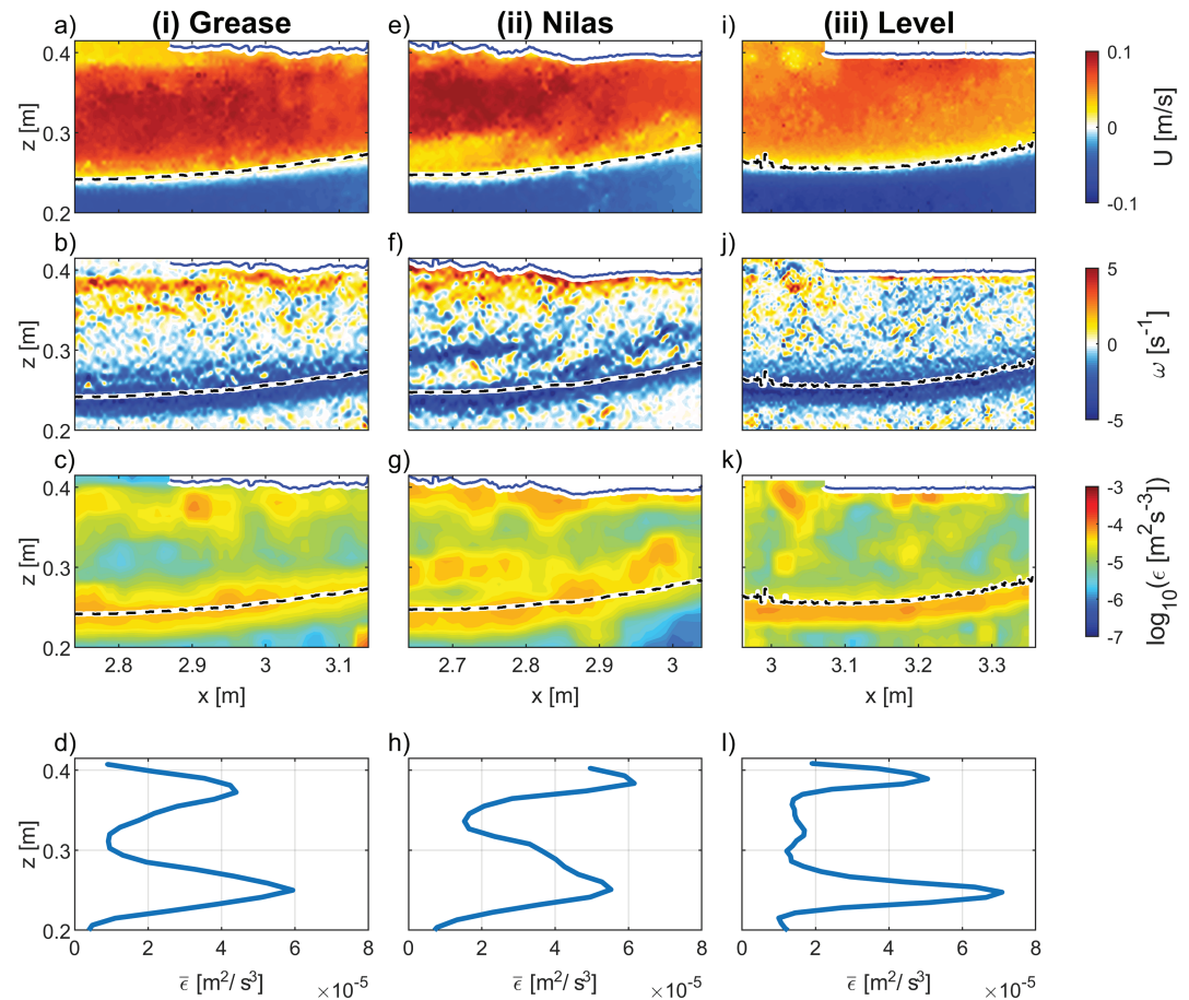
Figure 5. PIV measurements of (a, e, i) horizontal velocity u (m/s), (b, f, j) vorticity \omega ( s^{-1} ), and corresponding calculations of (c, g, k) TKE dissipation \log_{10}(\epsilon) ( m^2/s^3 ), and (d, h, l) mean TKE dissipation \bar{\epsilon} ( m^2/s^3 ) under (i) grease ice (a–d), (ii) nilas ice (e–h), and (iii) level ice (i–l). The black dashed line and the solid blue line depict the top of the pycnocline and the underside of the ice, respectively.
