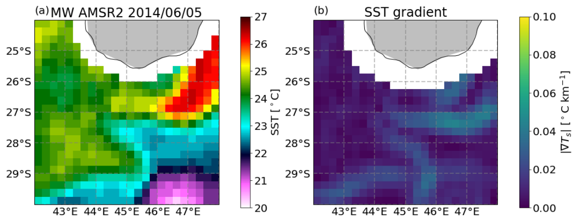
Figure A2. (a) SST captured by AMSR2 on the 5 June 2014, same date than SST shown in Figure 4 (b) Sobel gradient of SST captured by AMSR2.
