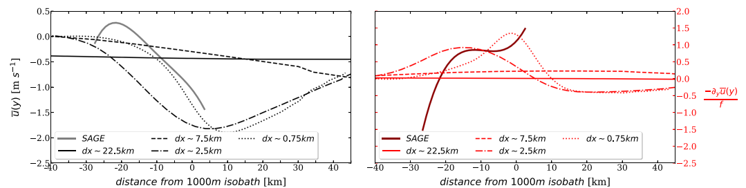
Figure 6. Cross-front sections of the mean along-front velocities ( \bar{u}(y) ) [ \text{m s}^{-1} ], left panel) and relative vorticity -\frac{\partial_y \bar{u}(y)}{f} , right panel at the SAGE location ( 25.75^\circ \text{ E} , shown in Figure 2a) for the SAGE glider data (Krug et al., 2017; gray and dark red lines) and for the four model nests at dx \sim 22.5 (plain lines), 7.5 (dashed-dotted lines), 2.5 (dashed lines), and 0.75 km (dotted lines) resolution. The bottom x-axis represents the cross-front distance from the 1000 m isobath, which represents the front position for the SAGE period. The highest-resolution nest has a frontal structure close to the SAGE dataset.
