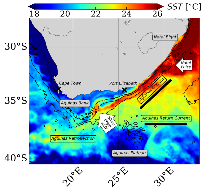
Figure 1. Snapshot of the Sea Surface Temperature (SST) [ ^{\circ} C] on 4 June 2014 from the Odyssea Regional South African product, showing the warm Agulhas Current extending from the southern boundary of the Mozambique Channel to the retroflexion and returning in the South Indian gyre as the Agulhas Return Current (black legends). The main topographic characteristics along the Agulhas path are displayed (gray legends). The thin black lines follow the 200, 1000, and 3000 m isobaths. Two perturbations, a Natal Pulse and a Shear-Edge eddy (white arrows), are developing along the Agulhas cyclonic front.
